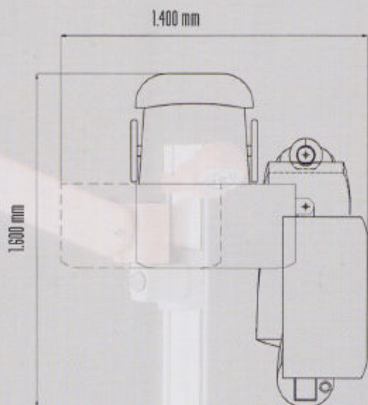
Dimensioni in mm. Dimensions in mm.
